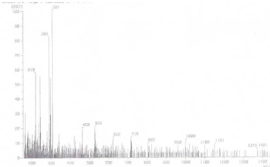
Figura C3. Complejo [\text{Cu}(\text{C}_{14}\text{H}_{10}\text{NO}_2\text{Cl}_2)_2]
