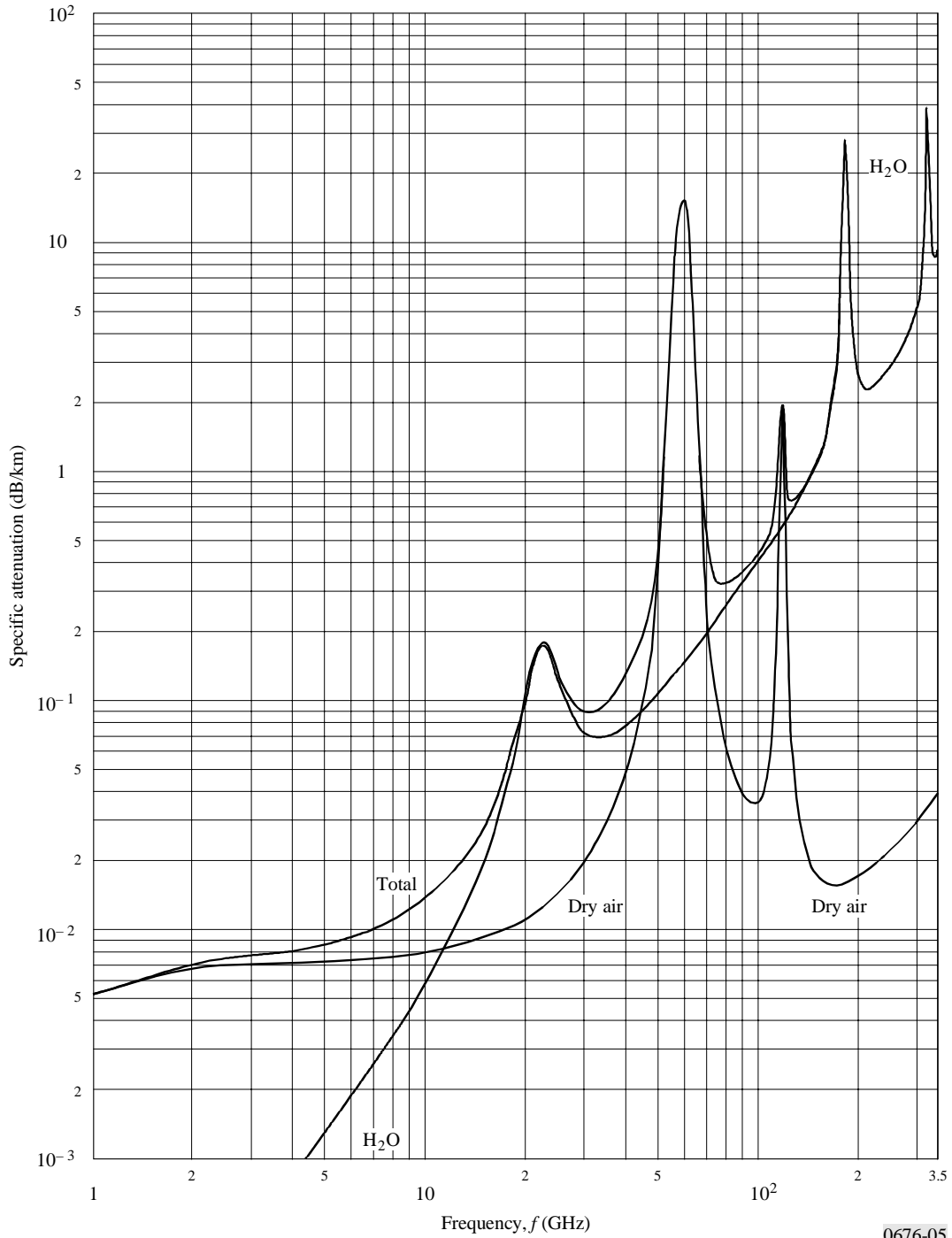
Specific attenuation due to atmospheric gases
