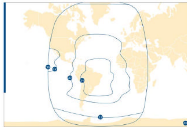
GLOBAL VERTICAL BEAM C-Band
