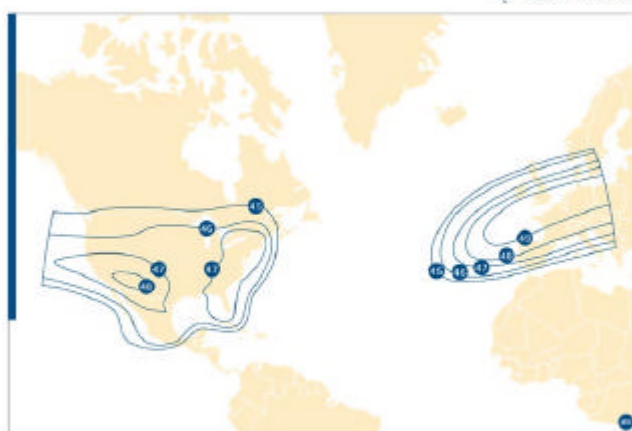
CONUS/EUROPE HORIZONTAL BEAM Ka-Band
