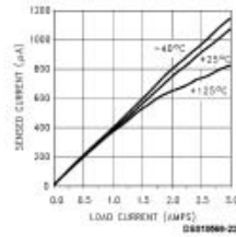
Current Sense Output vs Load Current
