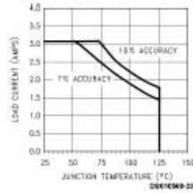
Current Sense Operating Region
