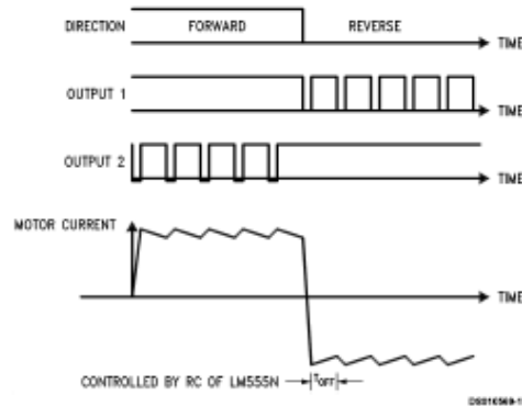
FIGURE 8. Switching Waveforms
