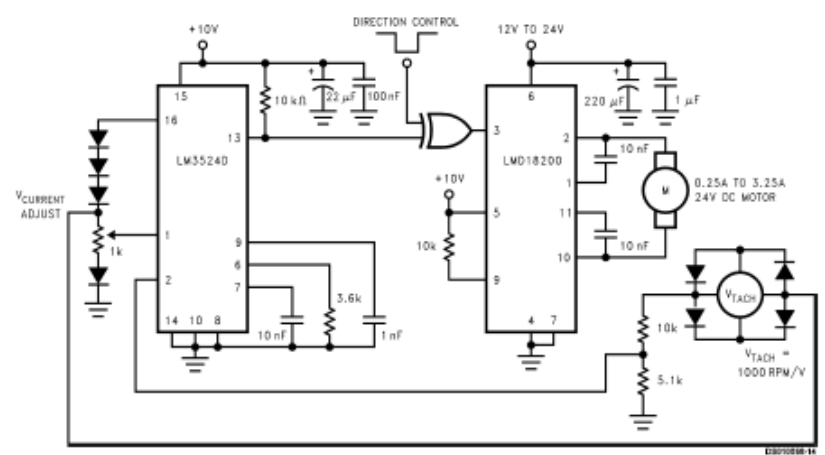
FIGURE 11. Regulate Velocity with Tachometer Feedback
