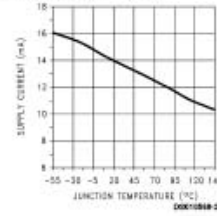
Supply Current vs Temperature (V D = 42V)
