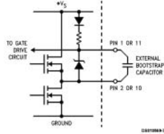
FIGURE 6. Bootstrap Circuitry
