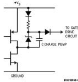
FIGURE 5. Internal Charge Pump Circuitry
