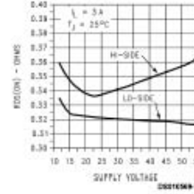
R DS(ON) vs Supply Voltage
