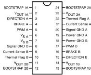
24-Lead Dual-in-Line Package Top View Order Number LMD18200-2D-QV 5562-5232501VXA LMD18200-2D/883 5562-5232501MXA See NS Package DA24B
