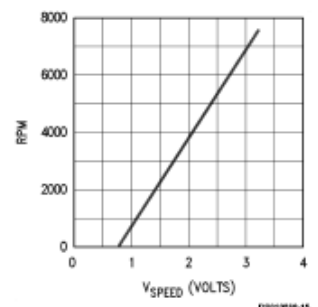
FIGURE 12. Motor Speed vs Control Voltage
