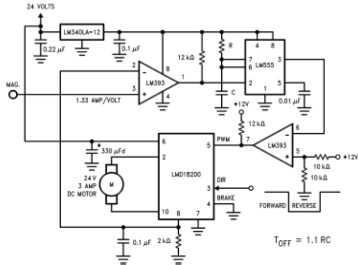
FIGURE 7. Fixed Off-Time Control
