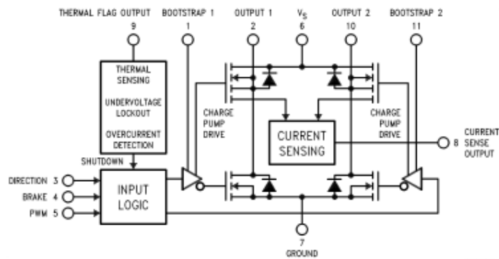
FIGURE 1. Functional Block Diagram of LMD18200
