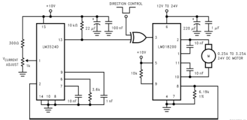
FIGURE 9. Locked Anti-Phase Control Regulates Torque
