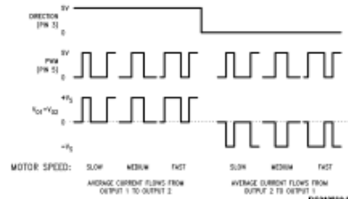
FIGURE 3. Sign/Magnitude PWM Control
