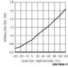
R DS(ON) vs Temperature
