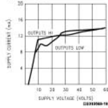
Supply Current vs Supply Voltage
