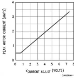
FIGURE 10. Peak Motor Current vs Adjustment Voltage
