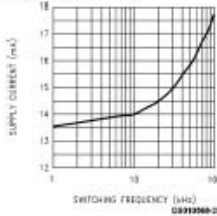
Supply Current vs Frequency (V D = 42V)
