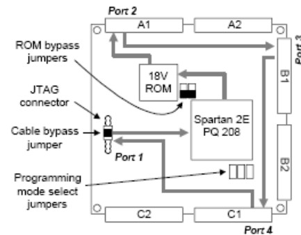
Figure 2. JTAG Signal Routing on D2-SB
