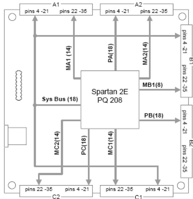
Figure 4. Expansion Connector Signal Routing
