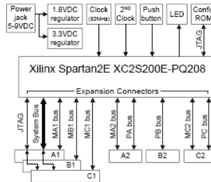
Figure 1. D2-SB Circuit Board Block Diagram
