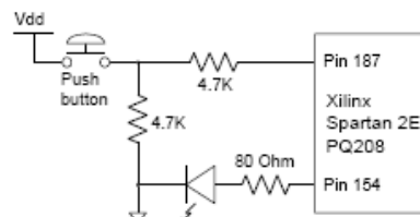
Figure 2. Pushbutton and LED Circuit
