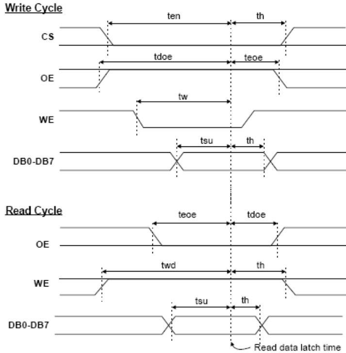
Figure 3. System Bus Timing
