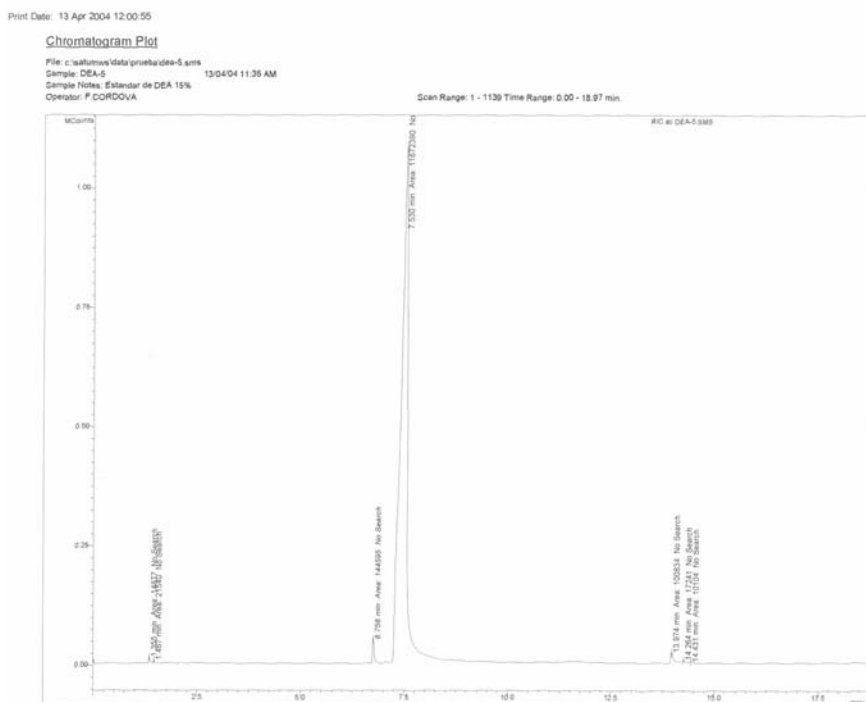
Figura J.8 Cromatograma de DEA
